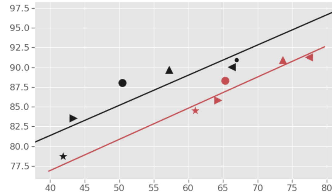
Cars
