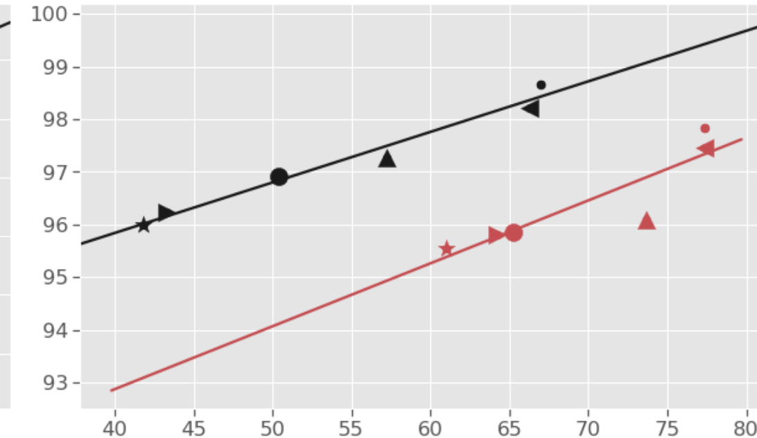
CIFAR-10
